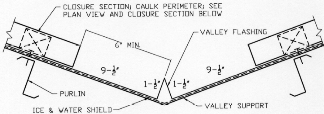
VALLEY DETAIL, SECTION A-A
