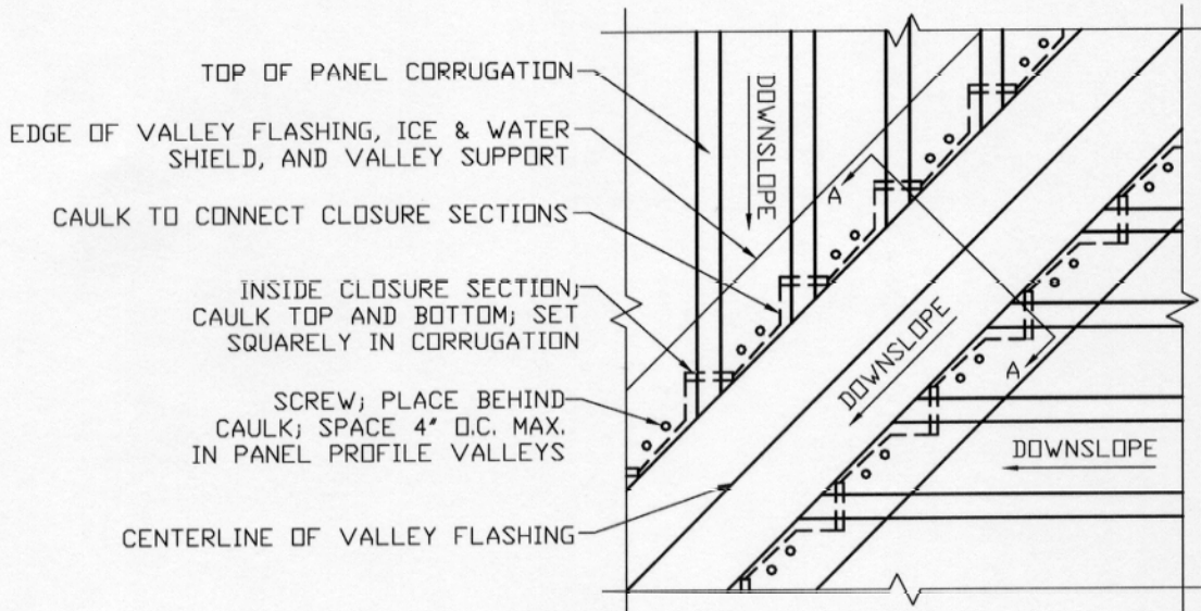
PLAN VIEW OF CLOSURES AND CAULK FOR EXPOSED FASTENER PANELS IN VALLEY
