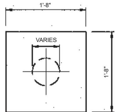
Flat Plate FSP-1
